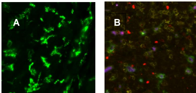
(A) CD63-CH015/anti-CH015-CL490, (B) UltraTag multiplex CD163/CD4/CD68/LAG3; primary and anti-hapten antibody staining @ 5 µg/mL; clones CD163 (EPR19518), CD4 (EP204), CD68 (68/684)/LAG3 (294)
